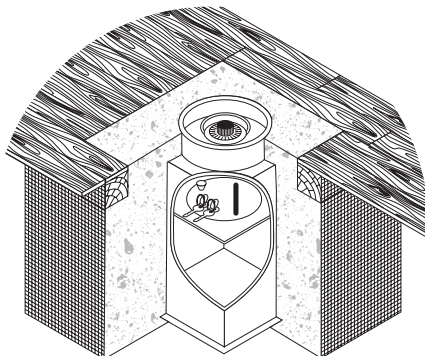
CUTAWAY VIEW OF STAR® DOUBLE COMPARTMENT INSTALLED IN CONCRETE
