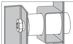
U SHAPE ANTI-PRY BOLT PROTECTOR
